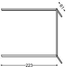
140 - 145 Venec omare Decorative architrave
